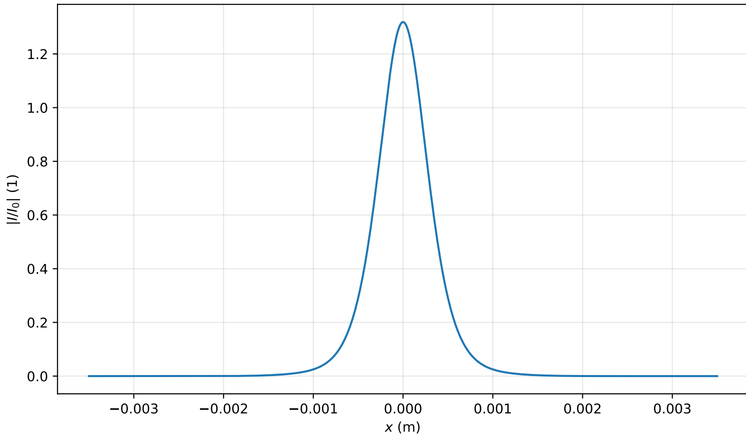
Intensity profile I(x, y = 0, z = 1.990m)/I_0 , P_{in}=0.8P_{cr} , artificial time
